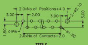
Recommended P. C. B Layout (Top Side)
