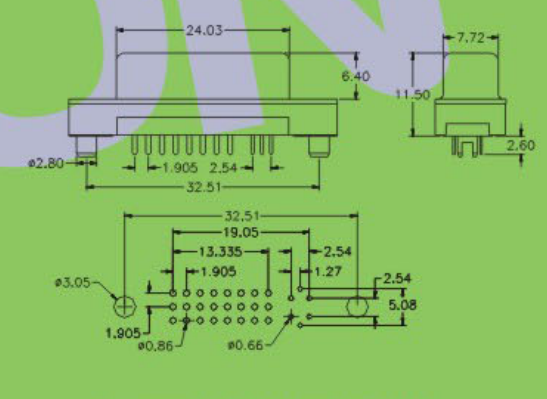
Recommended P. C. B Layout (Top Side)
