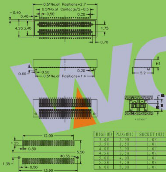
Recommended P.C.B Layout (Top Side)
