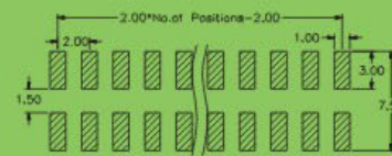
Recommended P.C.B Layout (Top Side)
