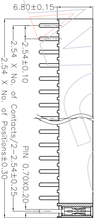
SECTION: B-B
