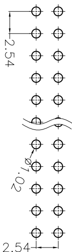
Recommended P.C.B Layout(TOP Side) (PCB BOARD TOLERANCE±0.05)
