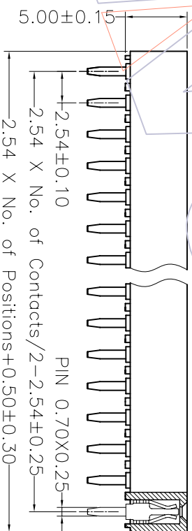
SECTION: B-B
