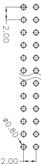
Recommended P.C.B Layout (Top Side) (PCB BOARD TOLERANCE±0.05)
