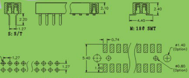
Recommended P. C. B Layout (Top Side)
