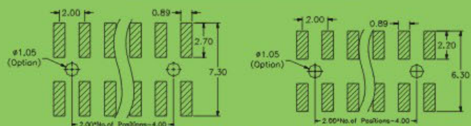
Recommended P. C. B Layout (Top Side)
